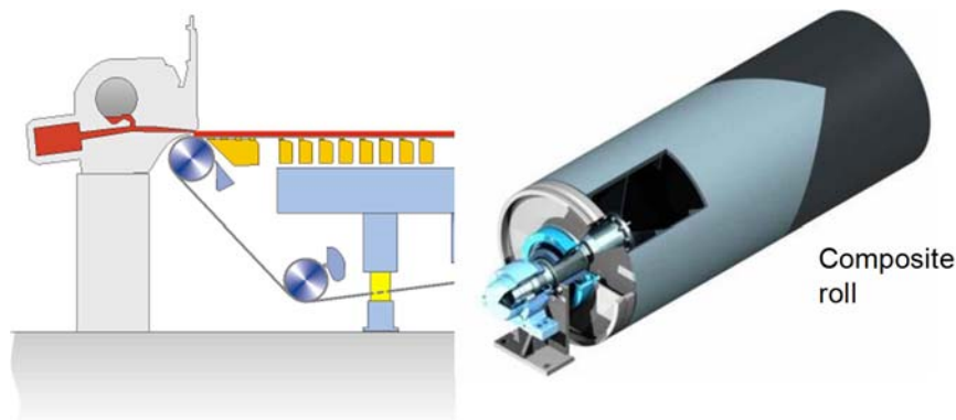
Figure 7. The breast roll may be replaced with a composite roll.
